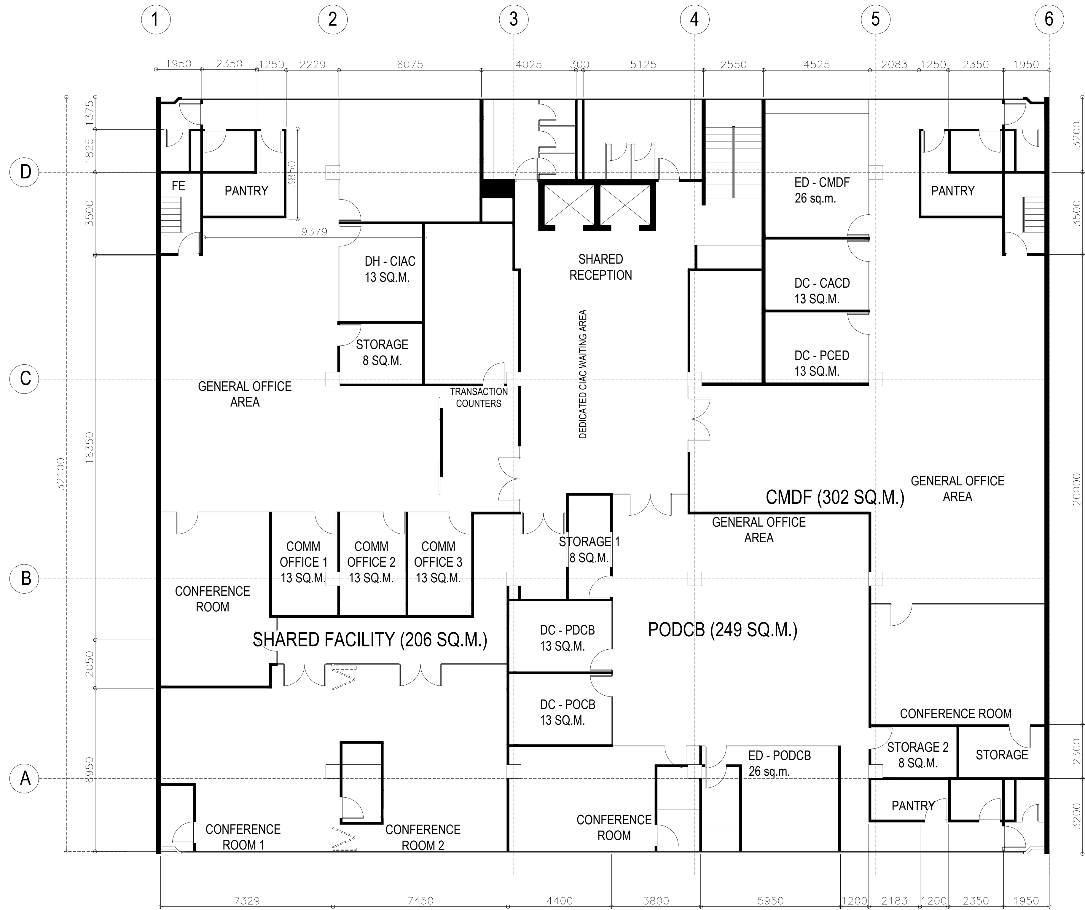
1 A 02 PROPOSED 2ND FLOOR LAY-OUT SCALE 1:100
