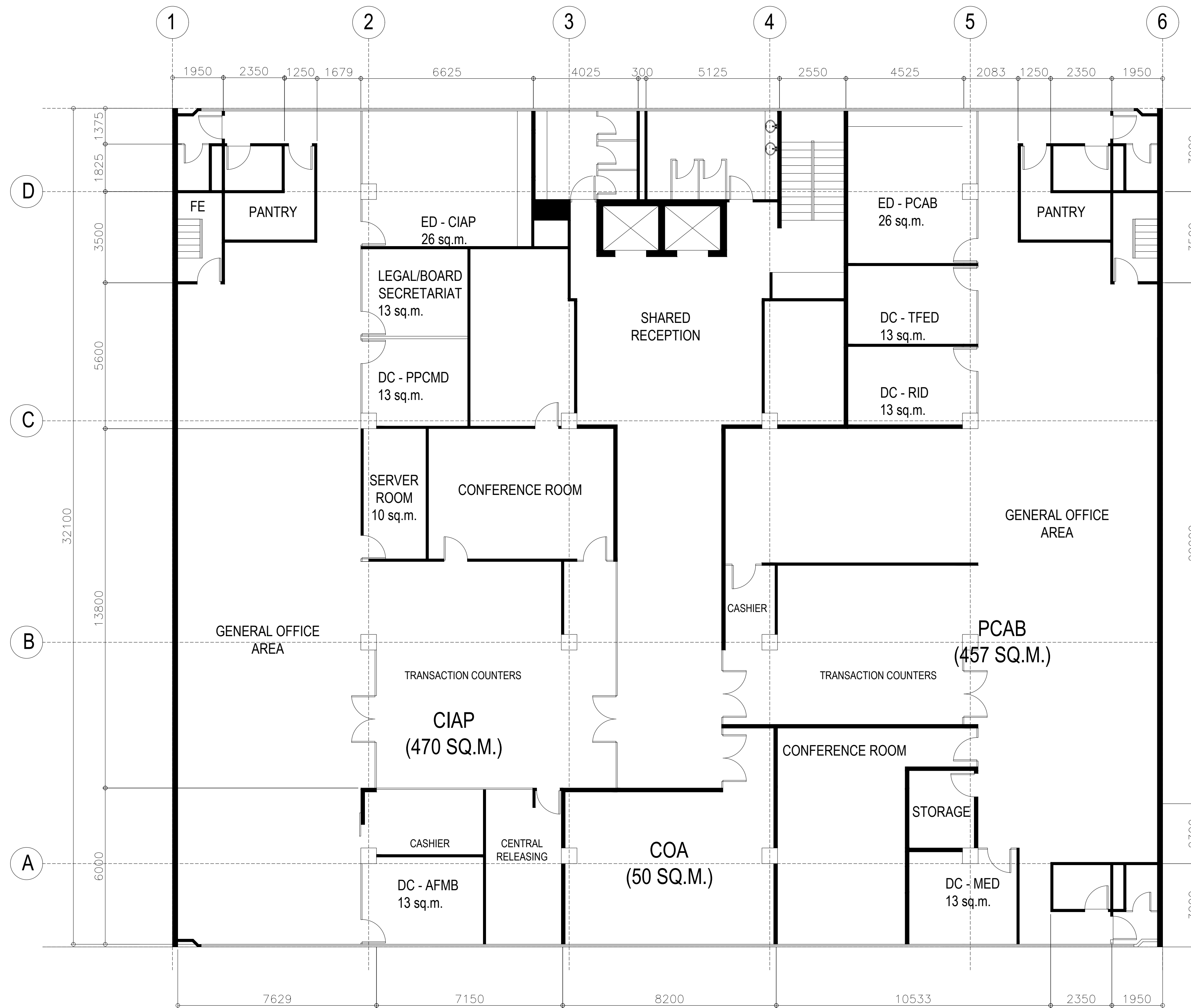
1 A 03 PROPOSED 3RD FLOOR LAY-OUT SCALE 1:100
